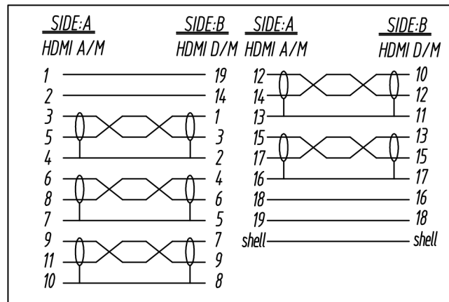
PIN OUT
